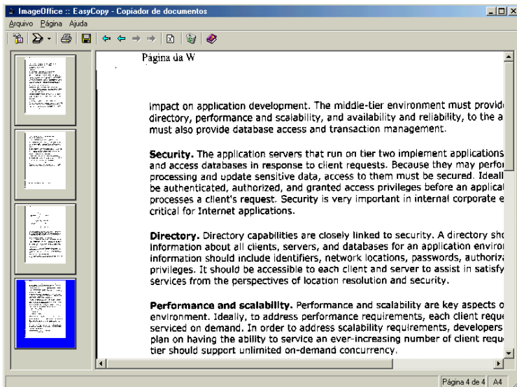
Figura 01 – Interface Principal
